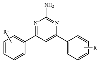
LC-MS analysis of aminopyrimidines (10).
