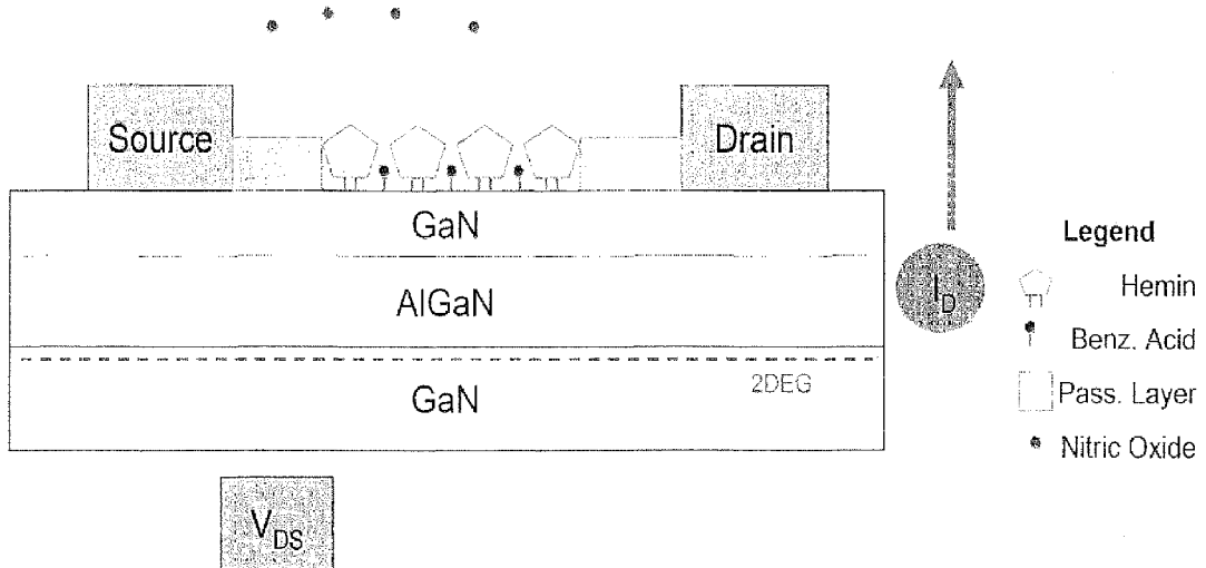
Schematic of Functionalized GaN-AlGaIn HFET
