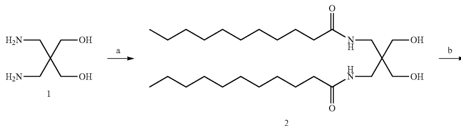
Scheme 1. Preparation of MNG Amphiphiles
