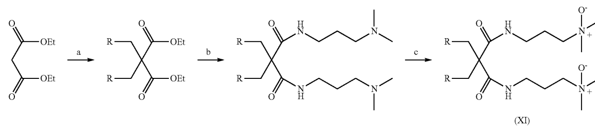
Scheme D. Preparation of Zwitterionic Amphiphiles
