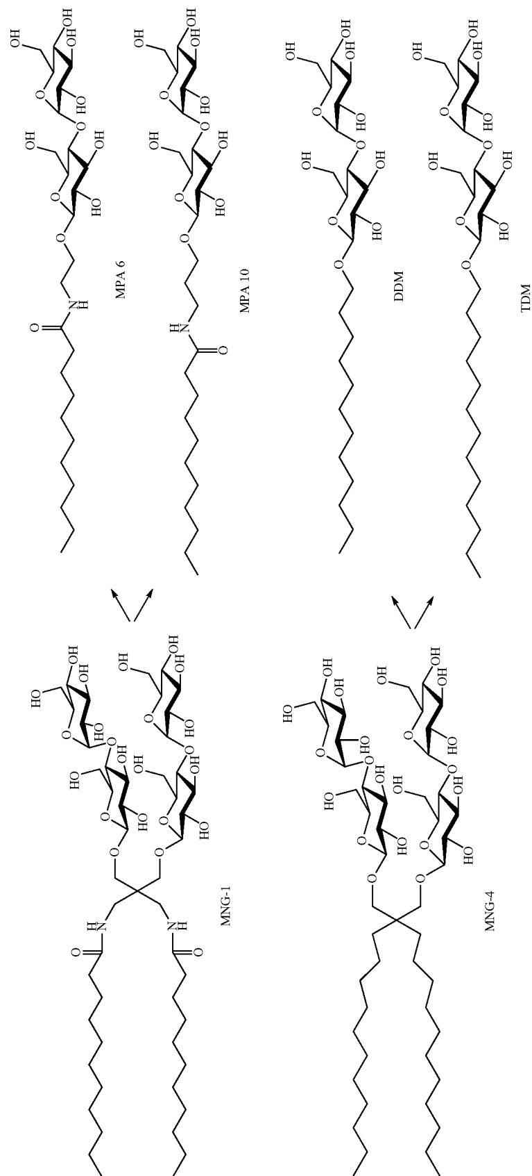
Scheme G. Specific MNG and MPA Amphiphiles
