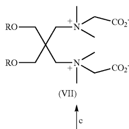
Scheme B. Preparation of Zwitterionic Amphiphiles
