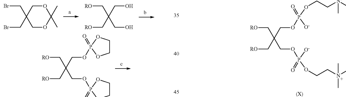
Scheme C. Preparation of Zwitterionic Amphiphiles
