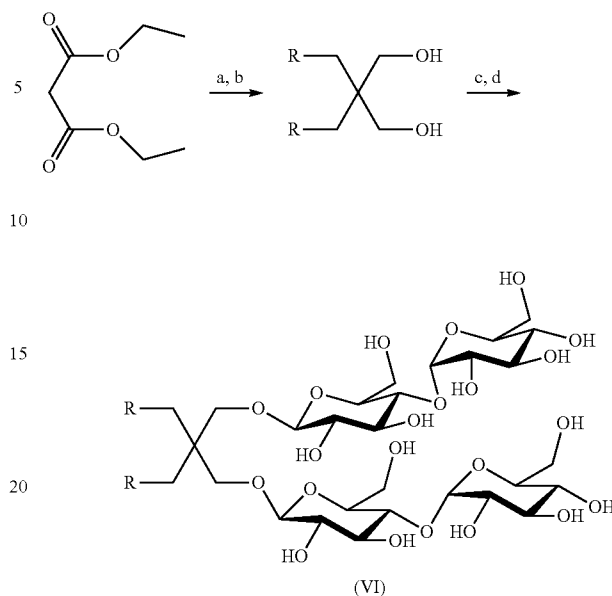
Scheme A. Preparation of Disaccharide Amphiphiles
