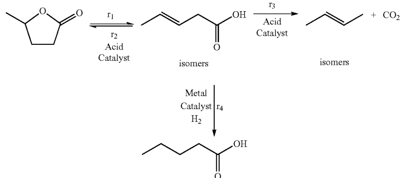
Scheme 3. Reactive pathway model
