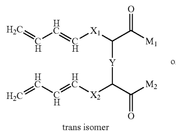
trans isomer
