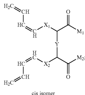
cis isomer
