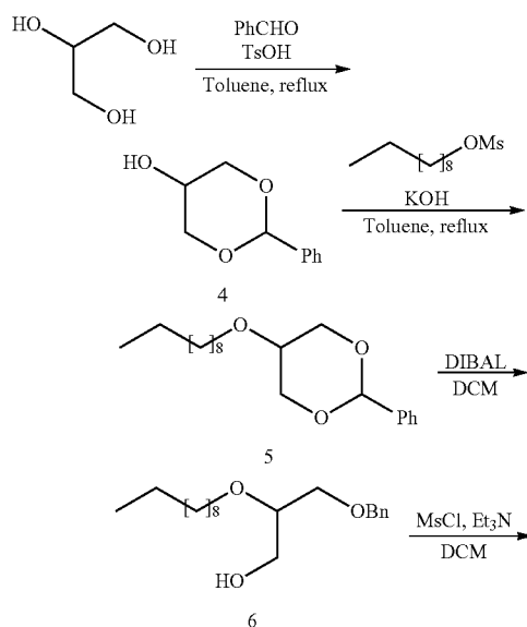
Scheme 2. Synthesis of mikroarm alcohols
