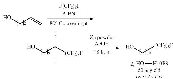
Scheme 1. Synthesis of linear and dibranched alcohols
