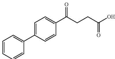
4-([1,1'-biphenyl]-4-yl)-4-oxobutanoic acid (4.3.10)
