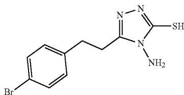
4-amino-5-(4-bromophenethyl)-4H-1,2,4-triazole-3-thiol (4.2.04)
