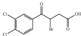
3-bromo-4-(3,4-dichlorophenyl)-4-oxobutanoic acid (4.4.02)
