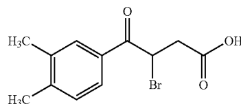
3-bromo-4-(3,4-dimethylphenyl)-4-oxobutanoic acid (4.4.03)
