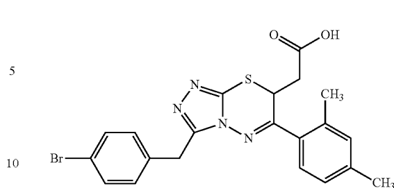
24 2-(3-(4-bromobenzyl)-6-(2,4-dimethylphenyl)-7H-[1,2,4]triazolo[3,4-b][1,3,4]thiadiazin-7-yl)acetic acid (4.5.11)
