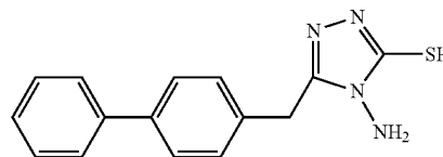
5-([1,1'-biphenyl]-4-ylmethyl)-4-amino-4H-1,2,4-triazole-3-thiol (4.2.06)
