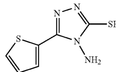
4-amino-5-(thiophen-2-yl)-4H-1,2,4-triazole-3-thiol (4.2.01)
