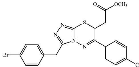
Methyl 2-(3-(4-bromobenzyl)-6-(4-chlorophenyl)-7H-[1,2,4]triazolo[3,4-b][1,3,4]thiadiazin-7-yl)acetate (14)
