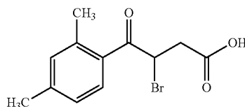
3-bromo-4-(2,4-dimethylphenyl)-4-oxobutanoic acid (4.4.09)
