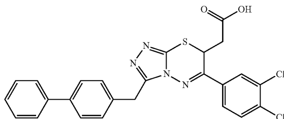
2-(3-([1,1'-biphenyl]-4-ylmethyl)-6-(3,4-dichlorophenyl)-7H-[1,2,4]triazolo[3,4-b][1,3,4]thiadiazin-7-yl)acetic acid (4.5.18)
