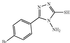
4-amino-5-(4-bromophenyl)-4H-1,2,4-triazole-3-thiol (4.2.03)
