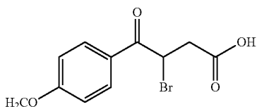
3-bromo-4-(4-methoxyphenyl)-4-oxobutanoic acid (4.4.07)
