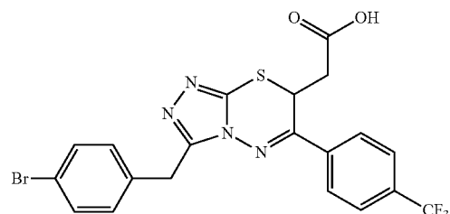
2-(3-(4-bromobenzyl)-6-(4-(trifluoromethyl)phenyl)-7H-[1,2,4]triazolo[3,4-b][1,3,4]thiadiazin-7-yl)acetic acid (20)
