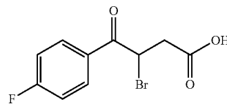
3-bromo-4-(4-fluorophenyl)-4-oxobutanoic acid (4.4.08)
