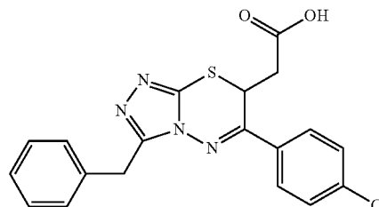
2-(3-benzyl-6-(4-chlorophenyl)-7H-[1,2,4]triazolo[3,4-b][1,3,4]thiadiazin-7-yl)acetic acid (4.5.15)
