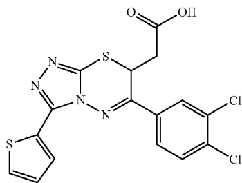
2-(6-(3,4-dichlorophenyl)-3-(thiophen-2-yl)-7H-[1,2,4]triazolo[3,4-b][1,3,4]thiadiazin-7-yl)acetic acid (18)
