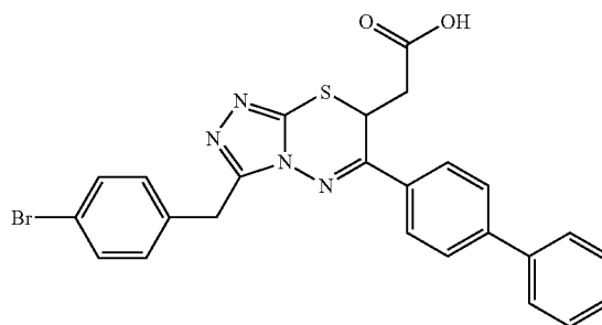
25 2-(6-([1,1'-biphenyl]-4-yl)-3-(4-bromobenzyl)-7H-[1,2,4]triazolo[3,4-b][1,3,4]thiadiazin-7-yl)acetic acid (4.5.12)
