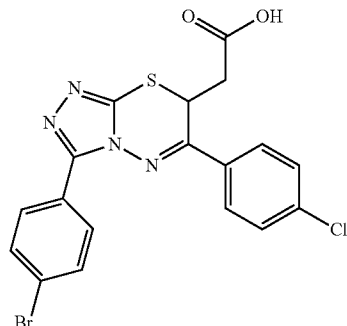
2-(3-(4-bromophenyl)-6-(4-chlorophenyl)-7H-[1,2,4]triazolo[3,4-b][1,3,4]thiadiazin-7-yl)acetic acid (4.5.13)
