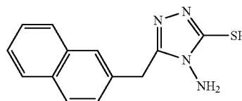
4-amino-5-(naphthalen-2-ylmethyl)-4H-1,2,4-triazole-3-thiol (4.2.07)
