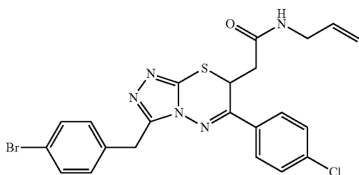
N-allyl-2-(3-(4-bromobenzyl)-6-(4-chlorophenyl)-7H-[1,2,4]triazolo[3,4-b][1,3,4]thiadiazin-7-yl)acetamide (35)
