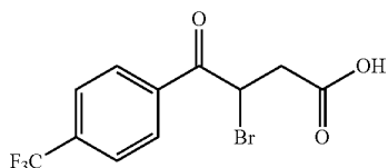
3-bromo-4-oxo-4-(4-(trifluoromethyl)phenyl)butanoic acid (4.4.05)
