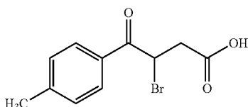
3-bromo-4-oxo-4-(p-tolyl)butanoic acid (4.4.06)
