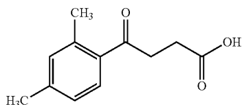
4-(2,4-dimethylphenyl)-4-oxobutanoic acid (4.3.09)
