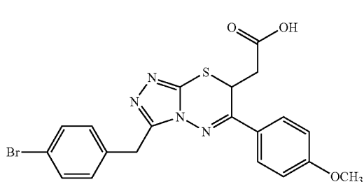
22 2-(3-(4-bromobenzyl)-6-(4-methoxyphenyl)-7H-[1,2,4]triazolo[3,4-b][1,3,4]thiadiazin-7-yl)acetic acid (22)
