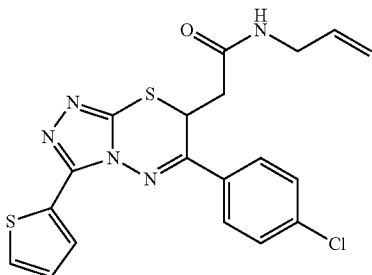
N-allyl-2-(6-(4-chlorophenyl)-3-(thiophen-2-yl)-7H-[1,2,4]triazolo[3,4-b][1,3,4]thiadiazin-7-yl)acetamide (34)
