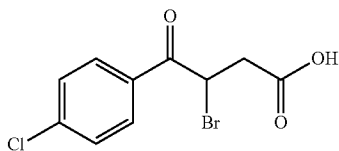
3-bromo-4-(4-chlorophenyl)-4-oxobutanoic acid (4.4.01)
